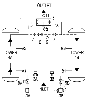
CDT40–CDT450 TOWER 4A DRYING TOWER 4B REGENERATING
