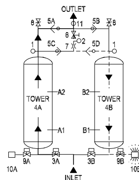
CDT590–CDT5400 TOWER 4A DRYING TOWER 4B REGENERATING
